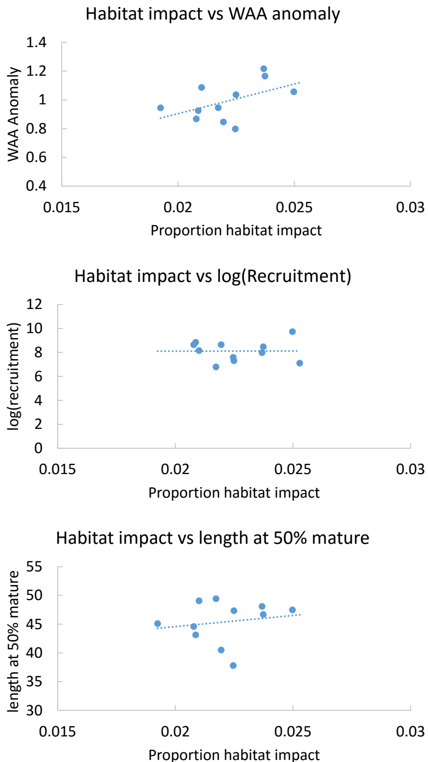
Figure 7 Correlations between annual habitat impact (2003-2014) in areas 610-630, and GOA pollock indicators for growth, recruitment, and maturation.
