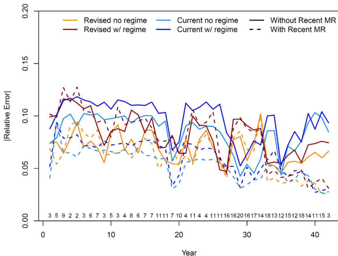
Figure 4. Median absolute values of relative error (expressed as proportional difference from the true value) through time in run reconstruction model estimates for 100 simulated time-series. Solid lines represent those in which the recent (2014-2017) mark-recapture estimates were not used in the run reconstruction model. Dashed lines represent scenarios in which the recent mark-recapture estimates were used in the run reconstruction model. Lines in orange shades represent results from the revised run reconstruction model, while blue shaded lines represent those from the current run reconstruction model. Darker shades of each color represent scenarios with population dynamics subject to regime shifts, while lighter shades represent scenarios without regime shifts. Numbers above x-axis indicate the number of escapement indices available each year, which are the same as in the real data set available for the Kuskokwim River.
