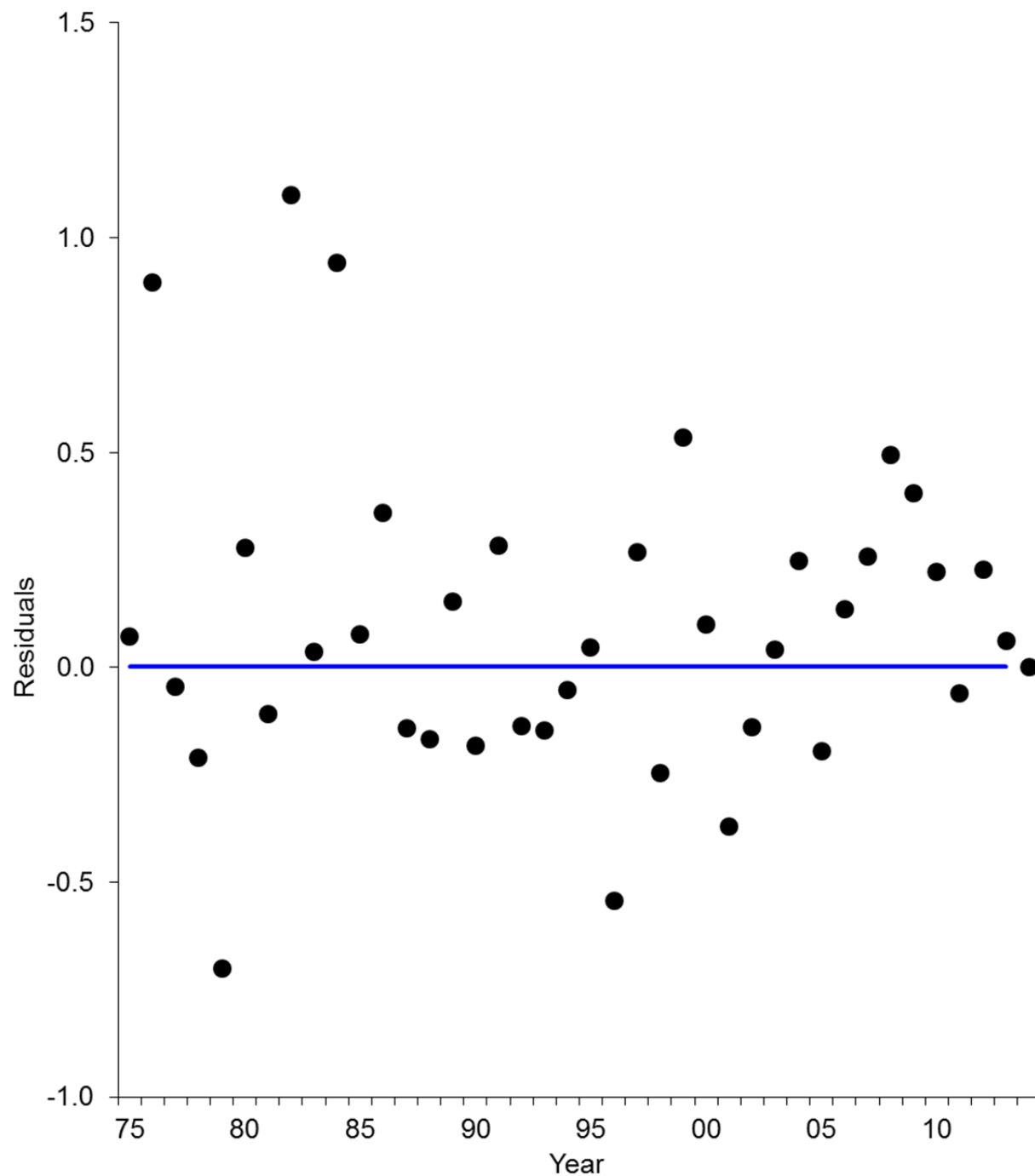
Figure 17(1a). Standardized residuals of total survey biomass under scenario 1a. Pot and trawl handling mortality rates were assumed to be 0.2 and 0.8, respectively.
