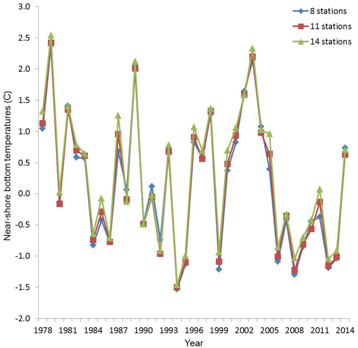
Figure B2. Mean near-shore bottom temperatures within 8, 11, and 14 NMFS survey stations around St. Matthew Island.
