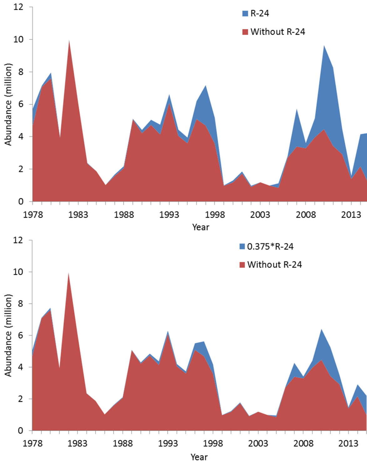
Figure 7. Comparisons of area-swept estimates of male (>89 mm CL) abundance without trawl survey station R-24, with reduction factor of 0.4 \cdot (401-25)/401 , or 37.5%, applied to station R-24, and without reduction factor applied to station R-24 for St. Matthew Island blue king crab.
