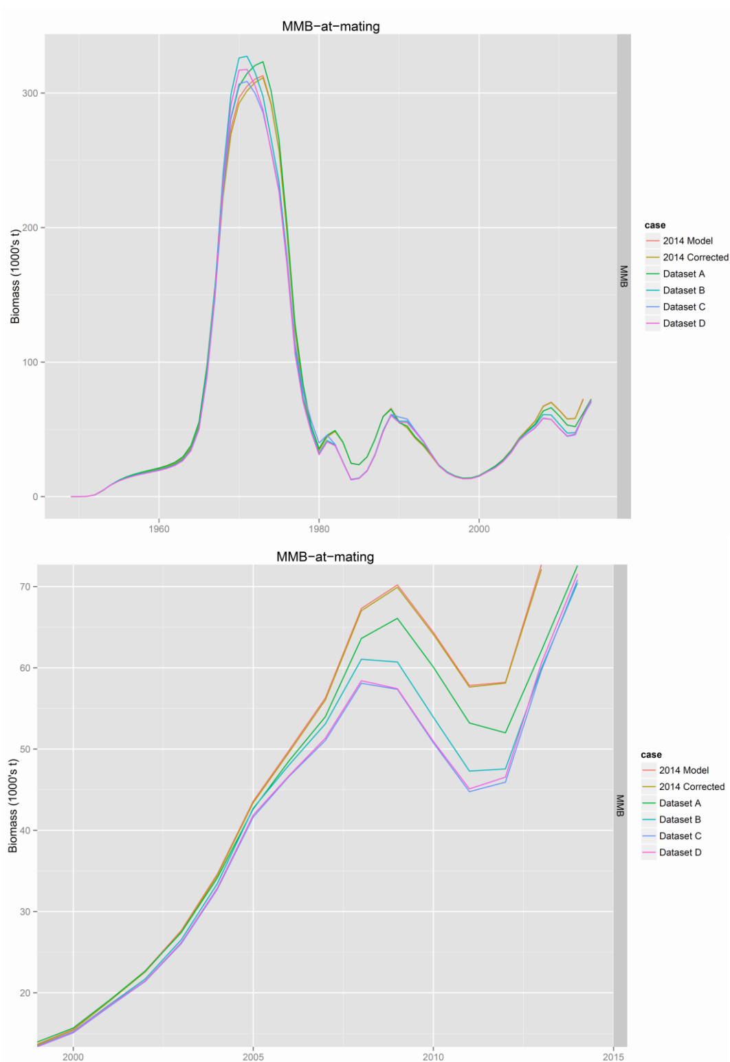
Figure 30. Estimated time series for MMB-at-mating from running Model A on the six datasets considered in the assessment, showing the incremental progression of data changes on model results. Upper graph: entire model time period. Lower graph: 1999-present.
