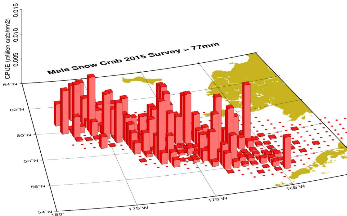
Figure 19. 2015 Survey CPUE (million crab per nm 2 ) of males > 77 mm by tow. Filled circles are tows with 0 cpue.
