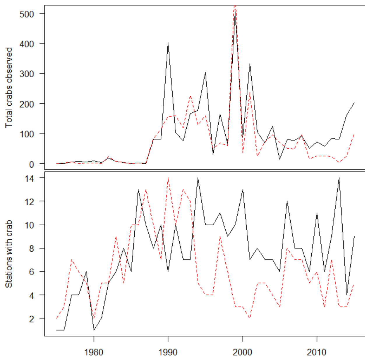
Figure 6. Total number of observed crab (top) and the number of stations that reported observations of crab (female = dashed line, male = solid line) from 1975-2014.
