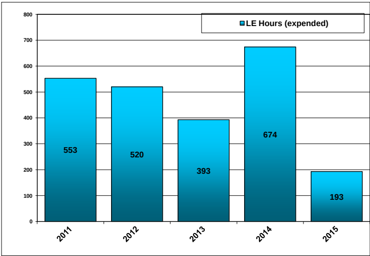
HC-130 Hours
