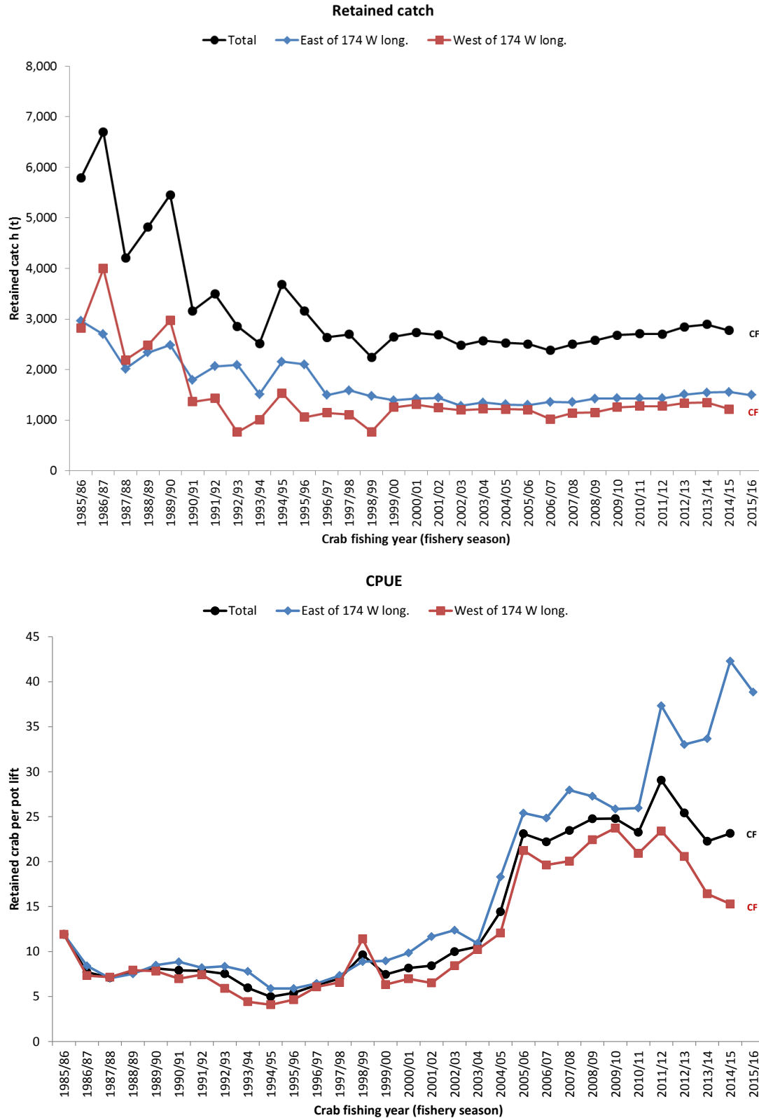
Figure 6. Retained catch (t; top) and catch per unit effort (CPUE; bottom) in the Aleutian Islands golden king crab fishery, 1985/86–2015/16: in the total area (east and west of 174° W longitude), in the area east of 174° W longitude, and in the area west of 174° W longitude. Note: CF = confidential.
