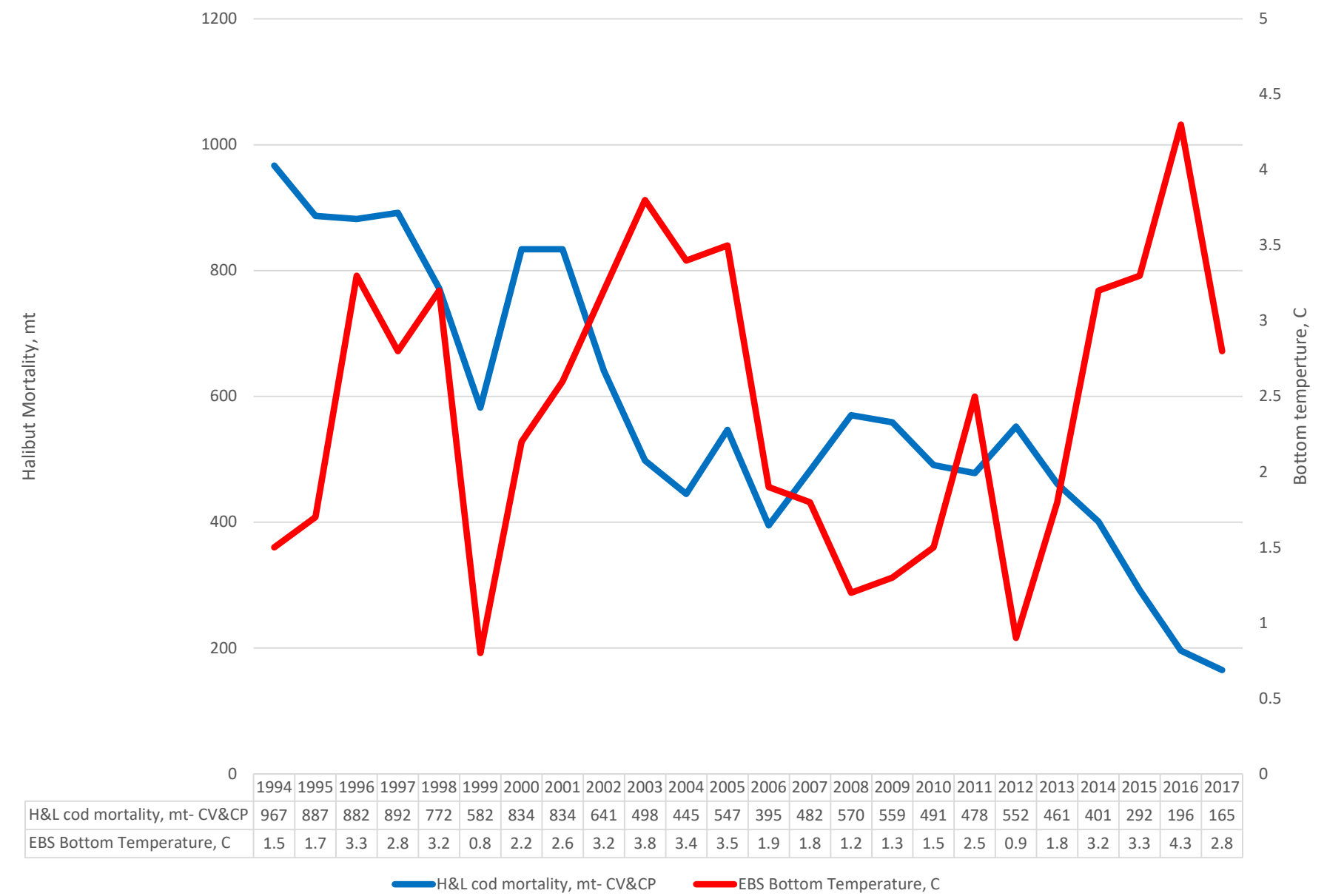
BSAI cod H&L halibut mortality and EBS bottom temperature, 1994-2017
